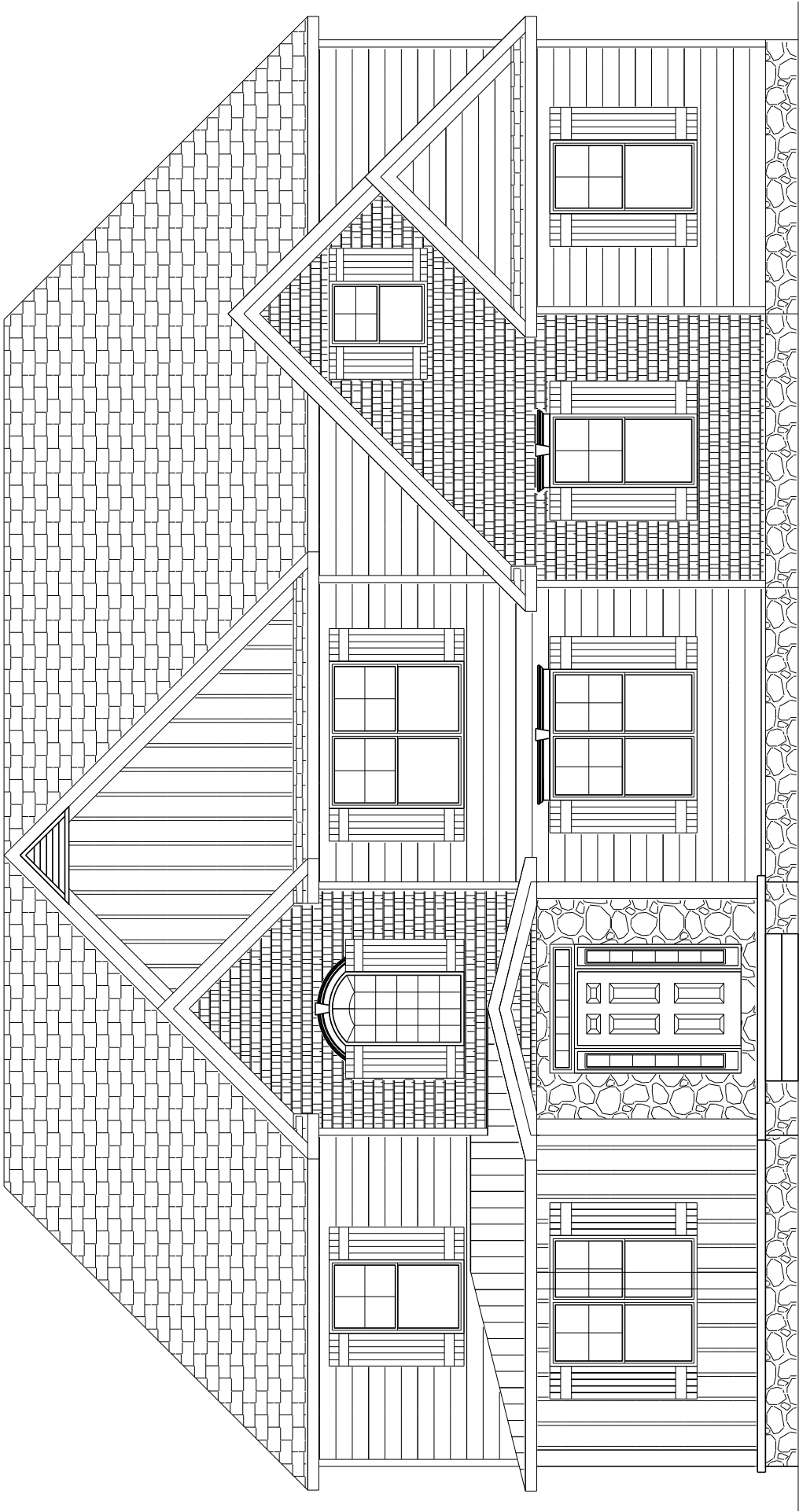
Front Elevation RB-215
